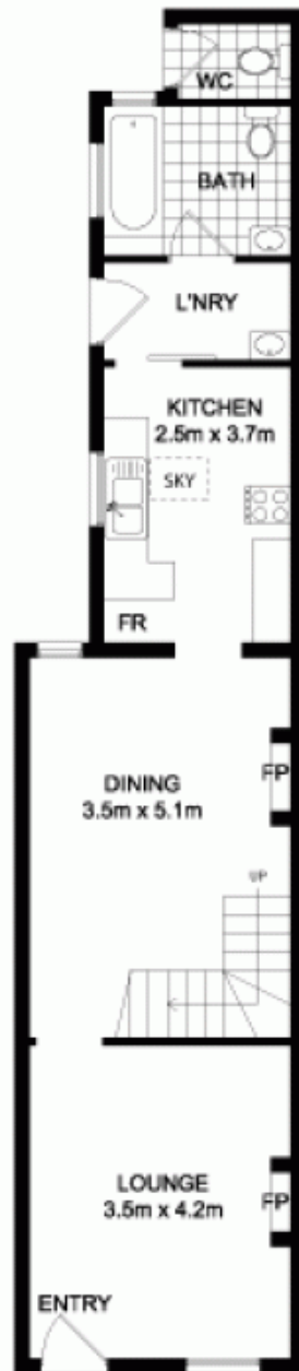
GROUND LEVEL
