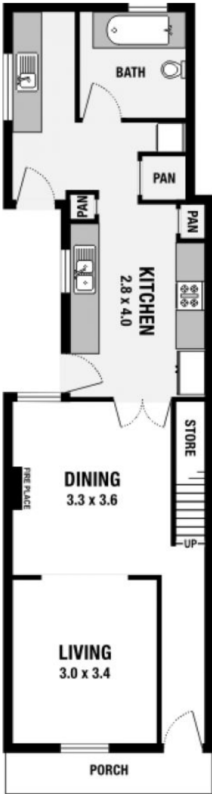
GROUND FLOOR
