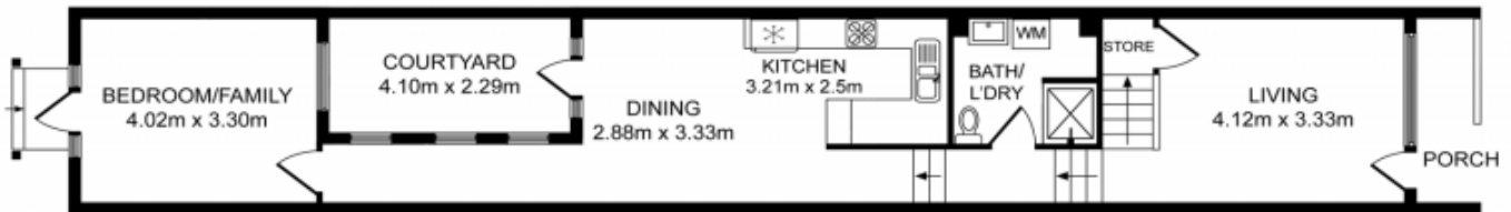
GROUND FLOOR
